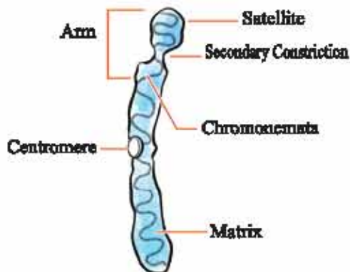
Figure : 2.11 Chromosome
