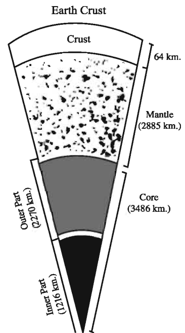
Fig. 3.1: Interior Structure Of the Earth
