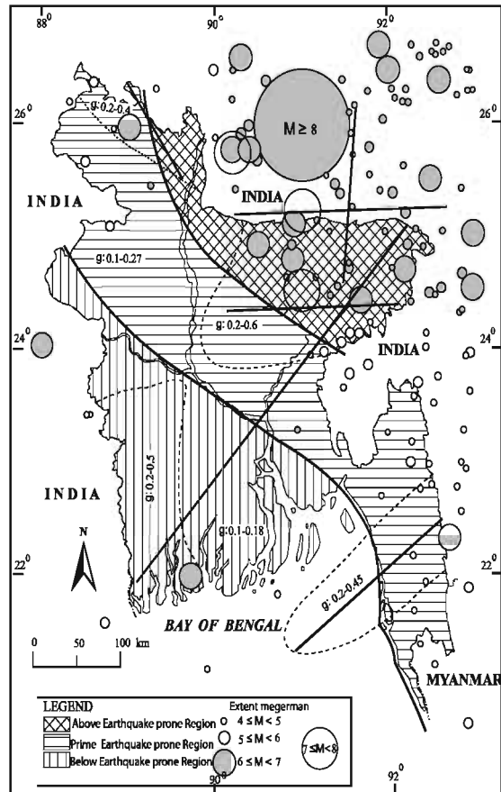
Figure 4.10: Earthquakes Prone Region of Bangladesh
