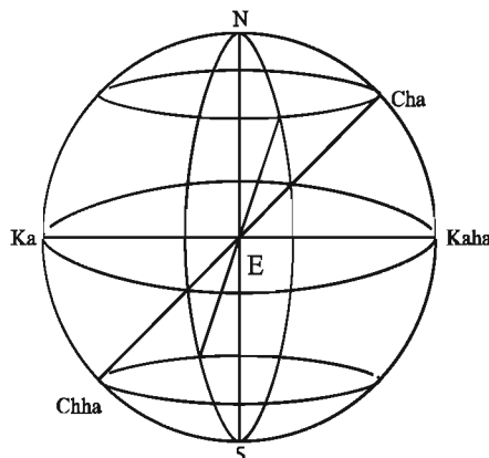
Figure 3.3 : The Antipodes Antipode of place Ka is Kaha Antipode of place Cha is Chha
