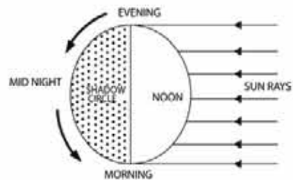
Figure 3.6: Occurrence of Day-night
