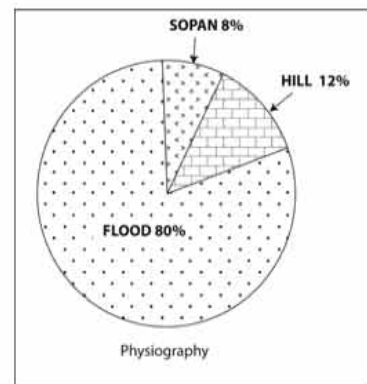
Figure 4.2 : Extent percentage of the Configuration of Land
