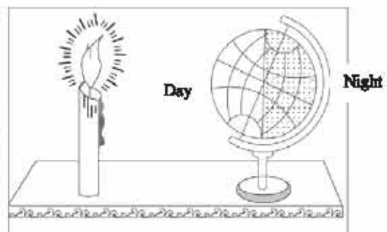
Figure 3.7 : With the candle and the globe
