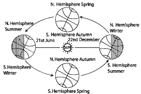
Figure 3.9 : The Change of seasons
